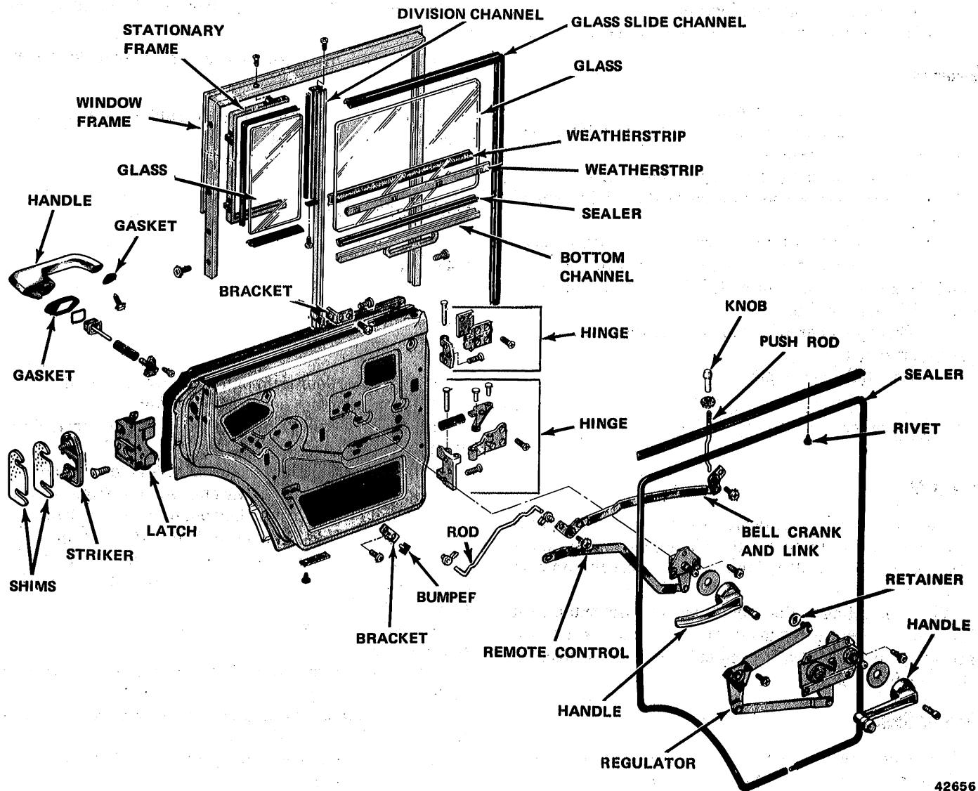
Fig. 3J-5 Rear Door—Cherokee-Wagoneer Models
