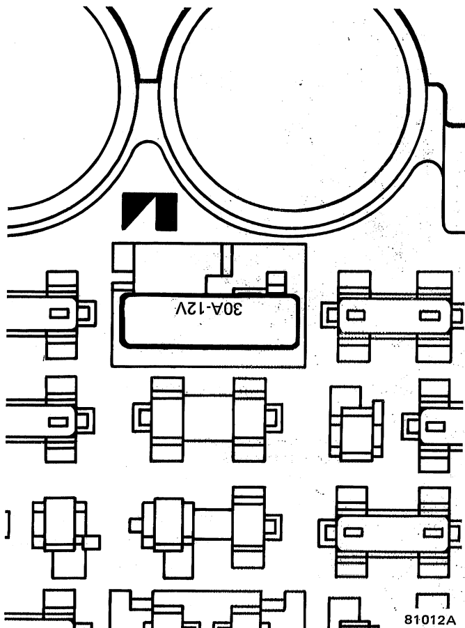
Fig. 3J-7 Circuit Breaker Location
