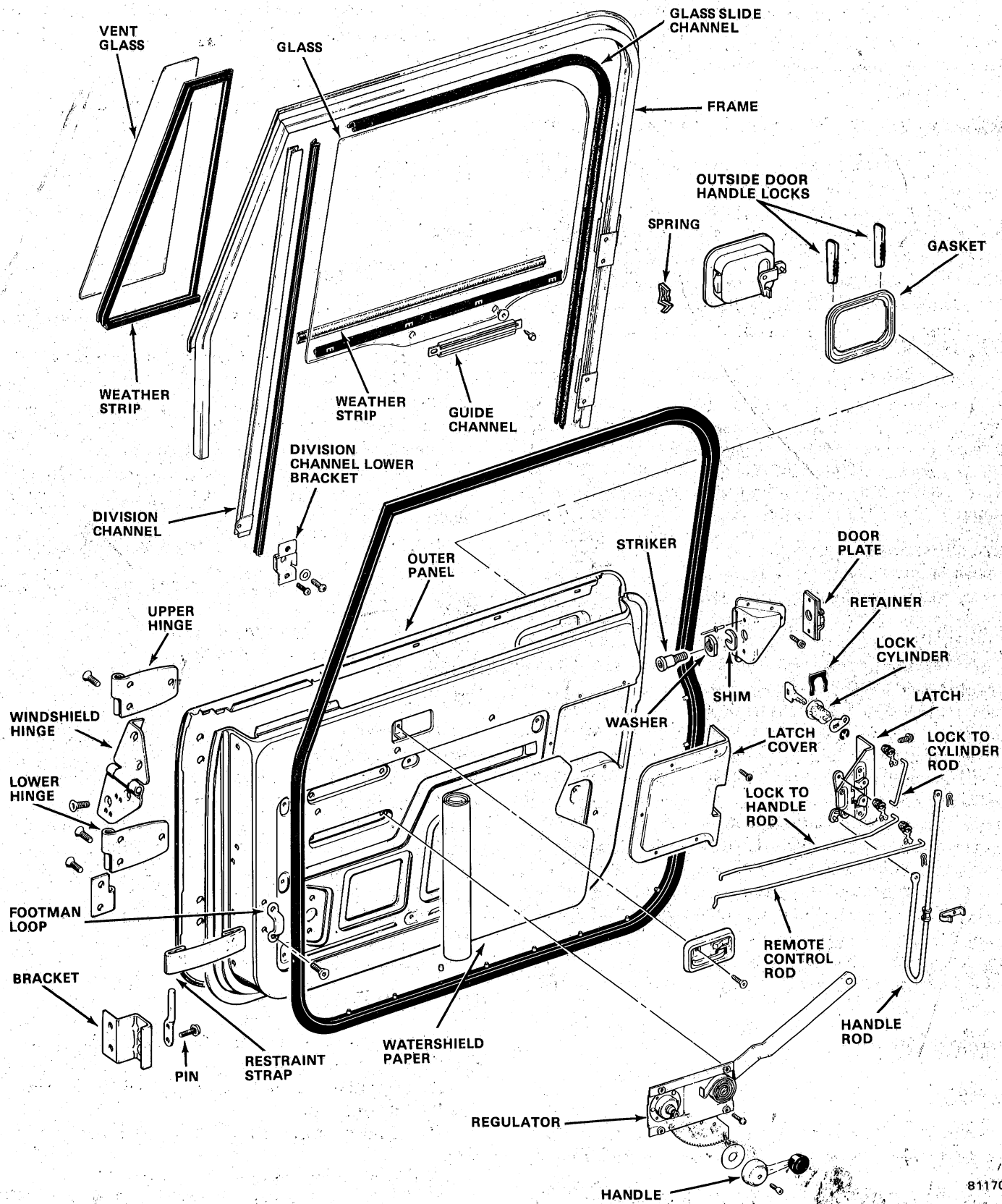
Fig. 3J-1 Front Door Exploded View—CJ and Scrambler Models
