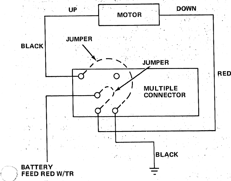
Fig. 3J-9 Motor Switch DOWN Test
